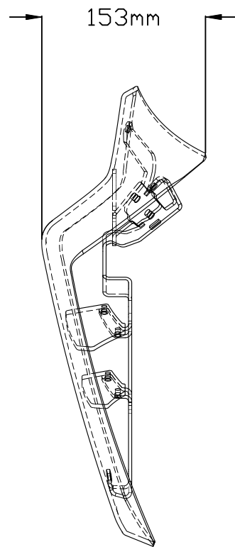
RIGHT SPOILER
